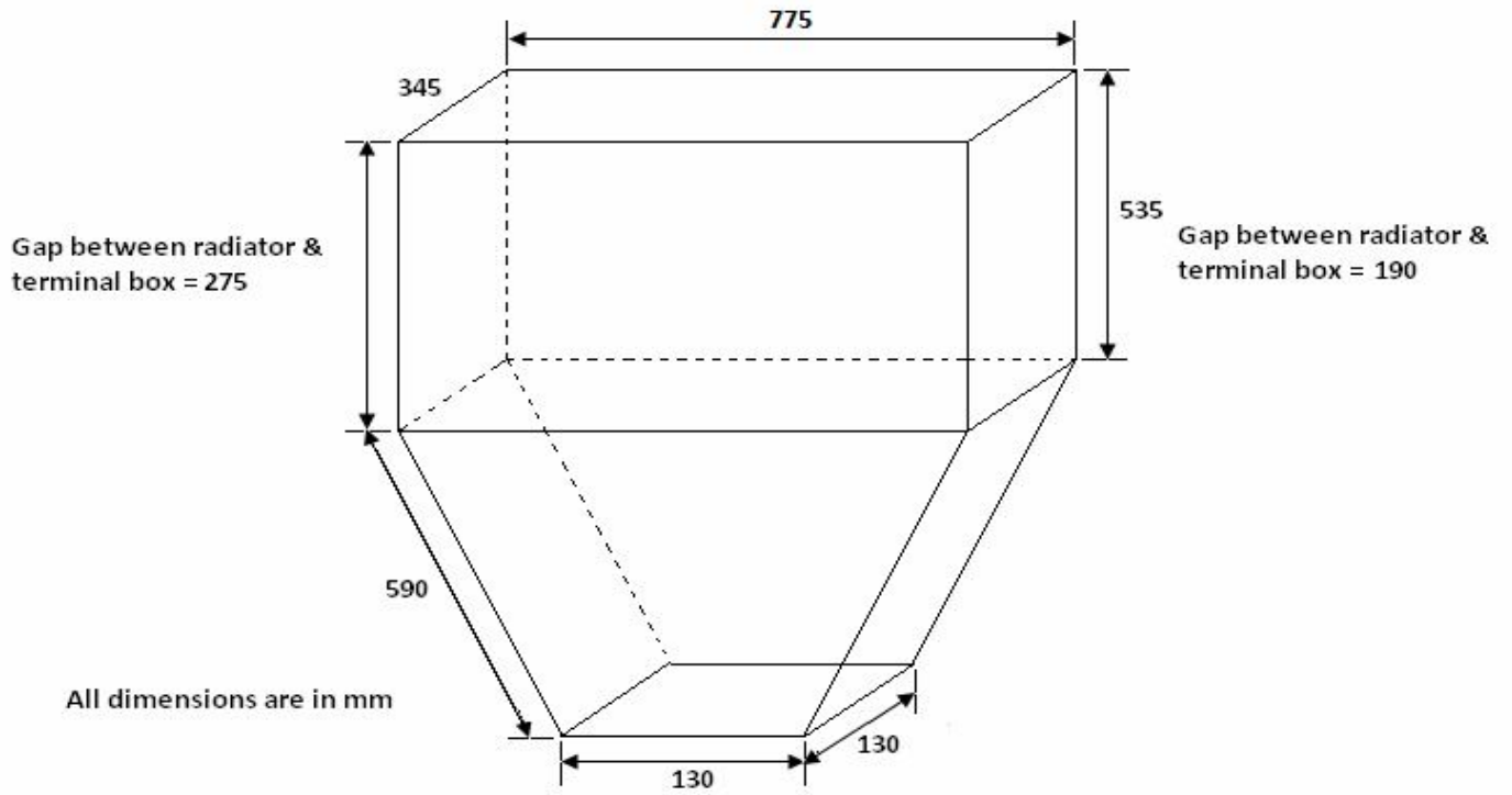
HV Terminal Box of 6 MVA 33 KV / 3.3 Transformaer of Master Control Sub-Station
