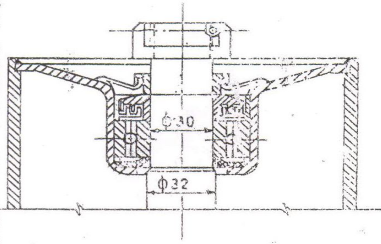
TYPICAL INTERNAL ARRANGEMENT (FOR REFERENCE ONLY)
