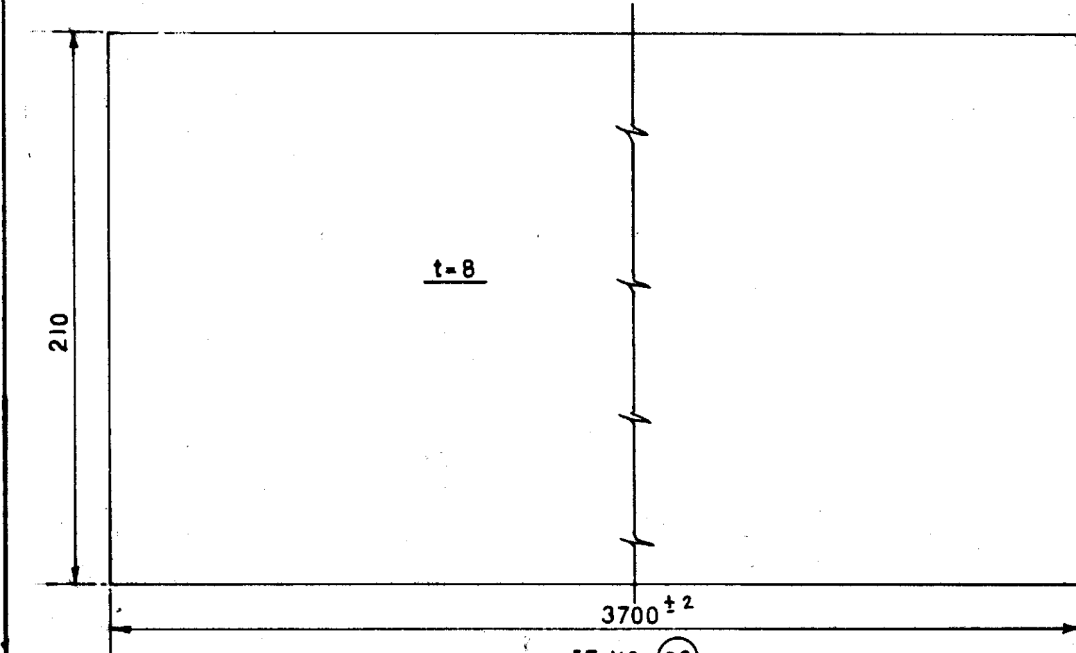
IT. NO. (05) WT=48.79 KG. (approx.)
