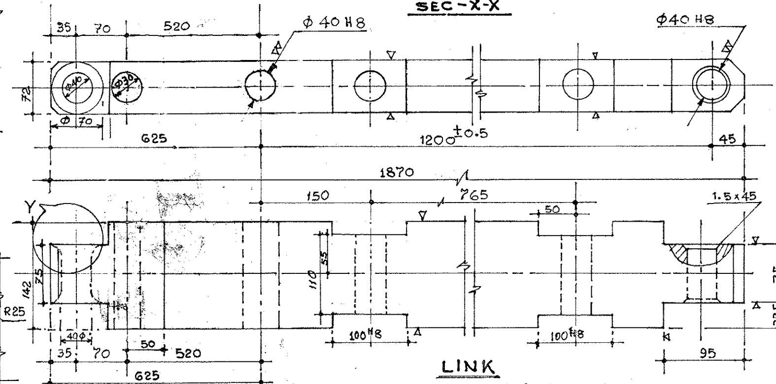
LINK WT. IN KG. = 32.64 KG. (approx.) DRG. NO. 210-085/5 SEC-X-X
