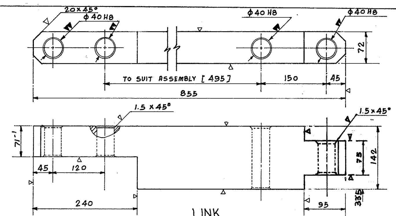
LINK WEIGHT-67.66 KG. (approx.) DRG. NO. 210-085/3 REF. BC1/04.00.00.04A 1. HOLES MARKED BY ▼ SHOULD BE DRILLED IN ASSEMBLY.
