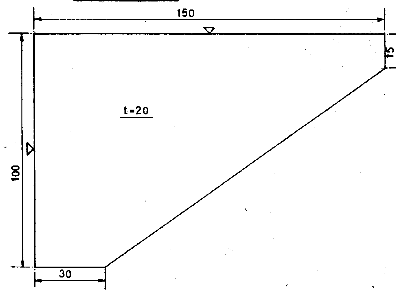
IT. NO. (16) WT. 1.55 KG. (approx.)
