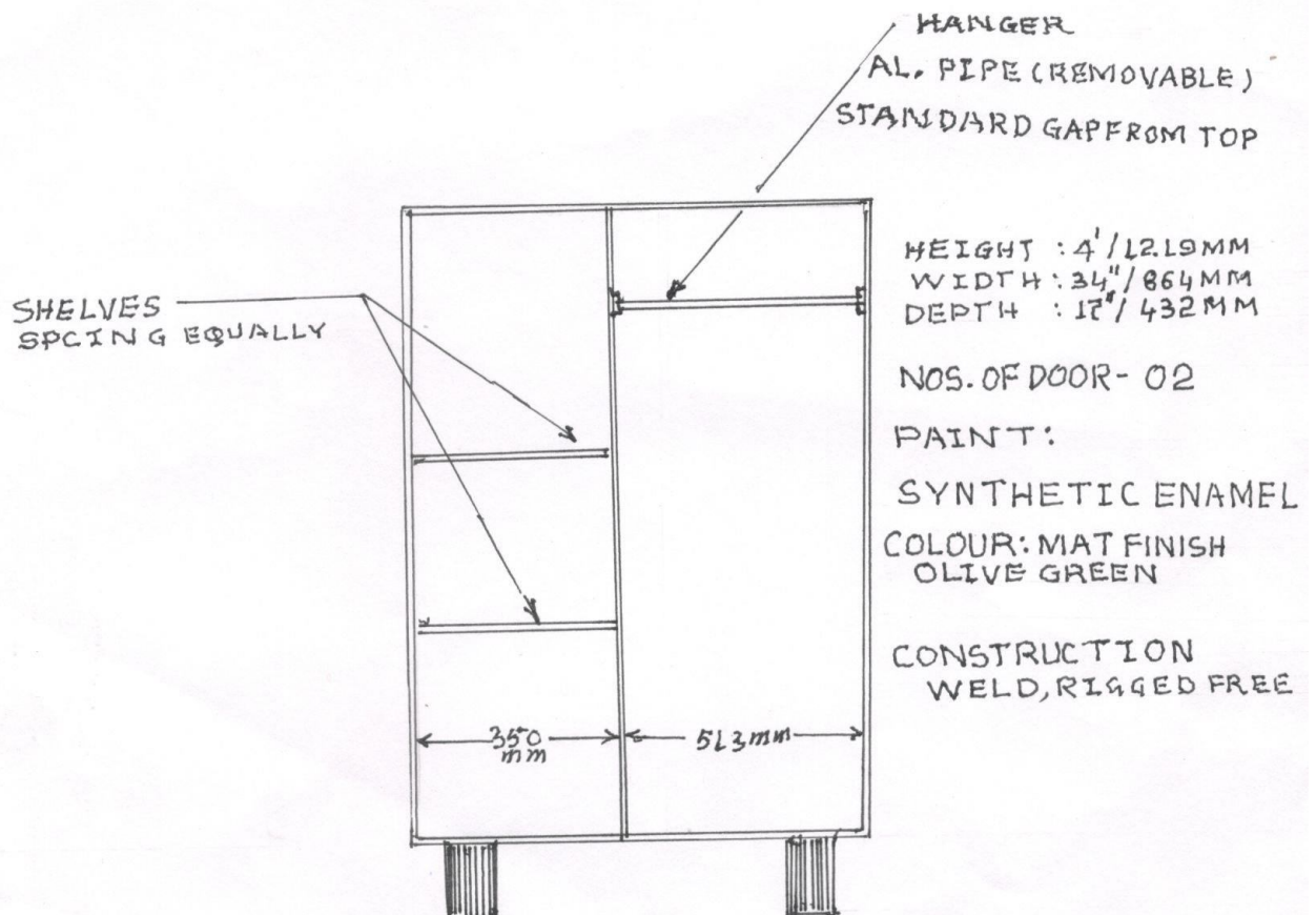
STEEL ALMIRAH, SHOWING THE LOCATION OF SHELVES & HANGER
